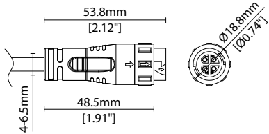
4 Pin LEDmix Female Connector IP67 (Premoulded)
